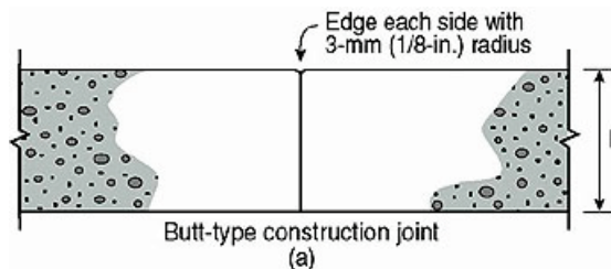
CONSTRUCTION JOINT – DIAGRAM 3
