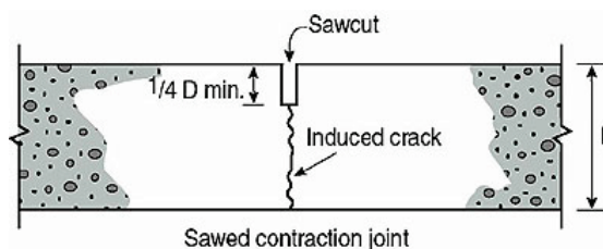
CONTRACTION JOINT – DIAGRAM 2
