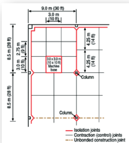
TYPICAL JOINT LAYOUT
